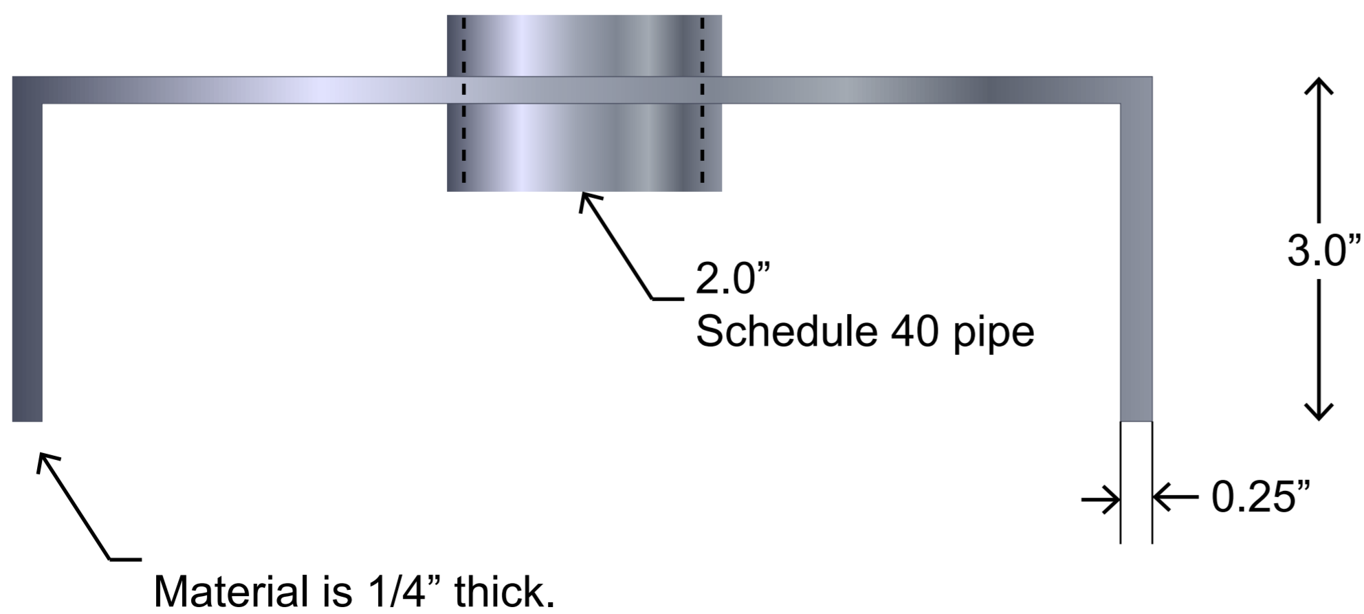
Side view
