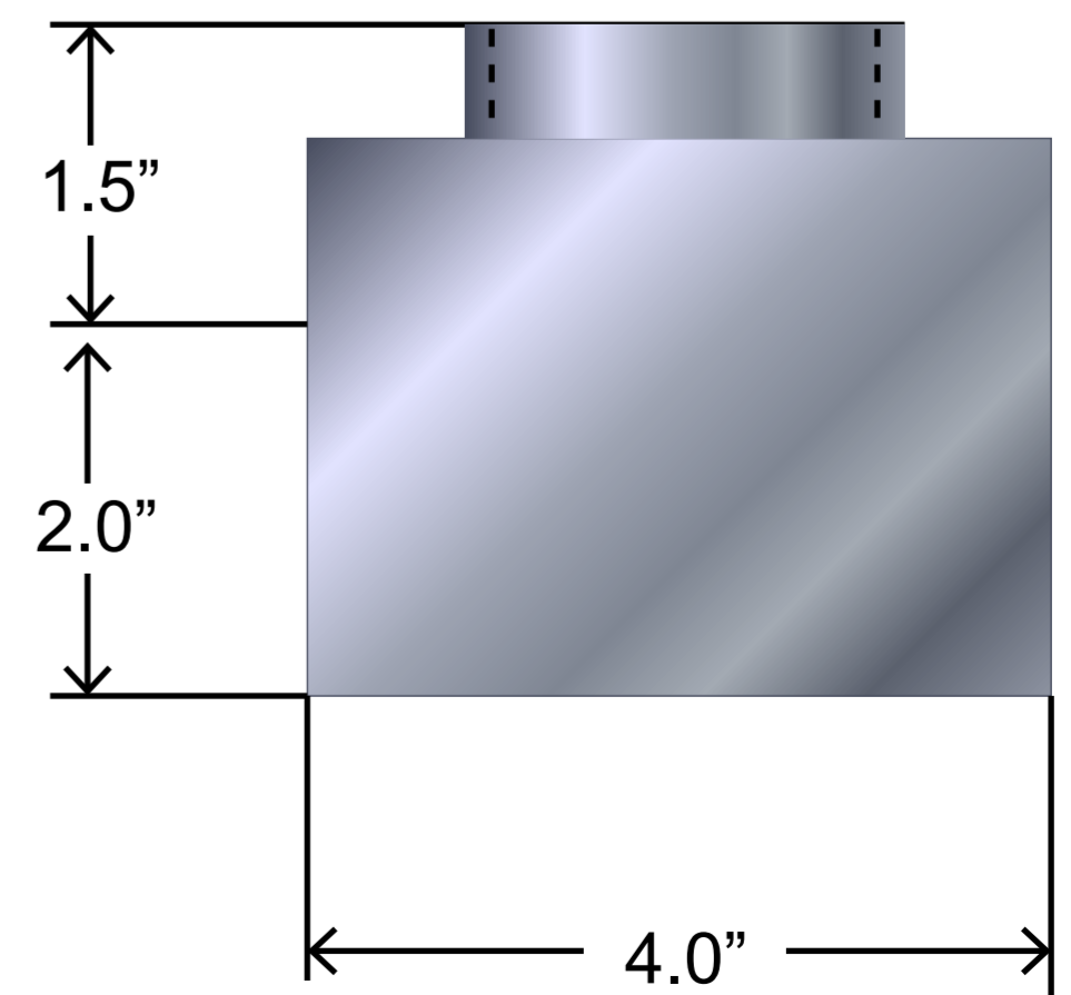
End view
